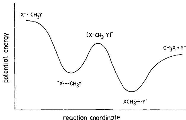
Figure 1. Reaction coordinate proposed by Brauman 3 for the gas-phase displacement reaction X^- + CH_3Y \rightarrow XCH_3 + Y^- .
